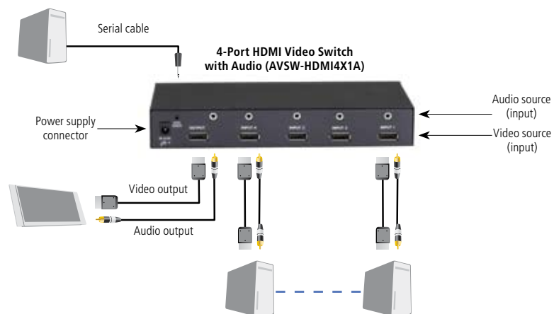
Figure 1. Back panel connections (AVSW-HDMI4X1A).
