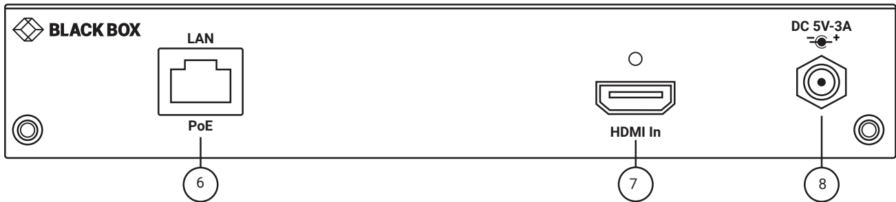
FIGURE 2-2. TRANSMITTER BACK PANEL
