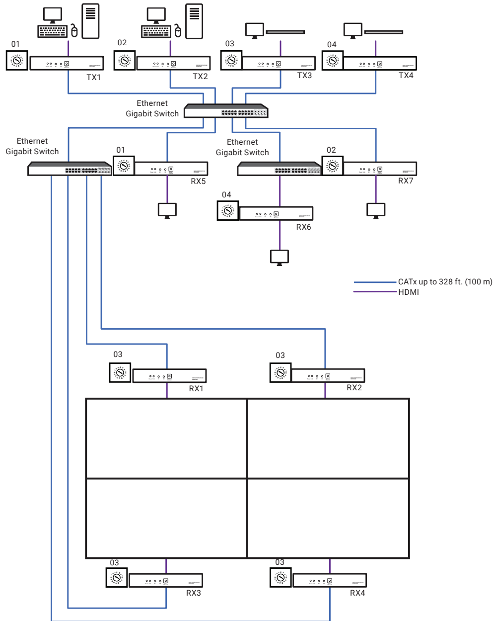
FIGURE 3-3. BROADCAST/CASCADE/MATRIX EXTENSION APPLICATION
